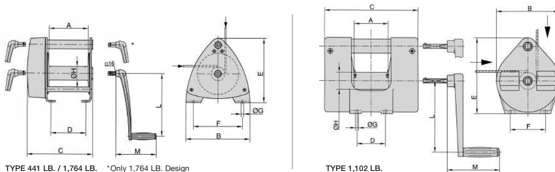
TYPE 441 LB. / 1,764 LB. *Only 1,764 LB. Design
