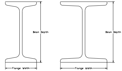
American Standard I-Beams Flange Slope 9° 27' - 44" Bevel 2 in 12
