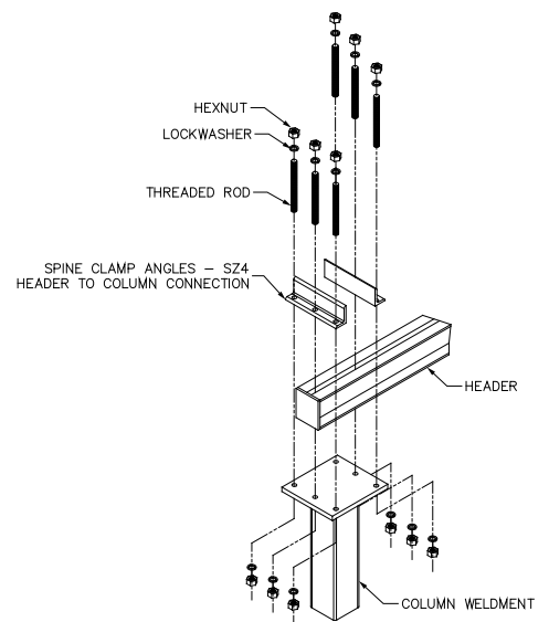
Diagram 3C. Installing header weldments on 6-bolt column cap plates.
