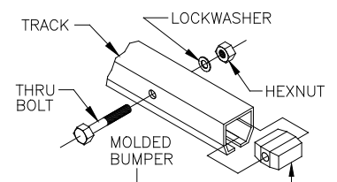
Diagram 5E. Installing end stop.
