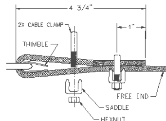
Diagram 9D. Saddling the cable on one end.
