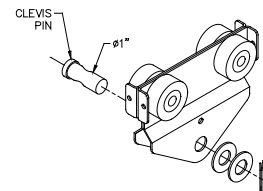
Diagram 6C. Installing hoist on 1000-2000# hoist trolley.
