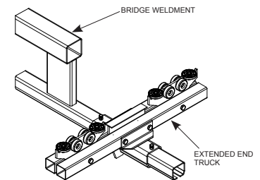
Diagram 5D. Installing extended clamping end truck. See NOTE .
