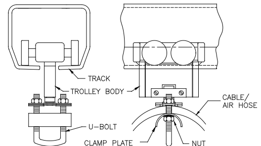
Diagram 8G. Installing electric cable or air hose on festoon trolley.
