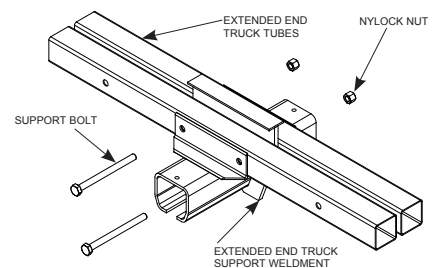
Diagram 5B. Assembling extended end truck.
