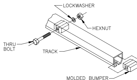
Diagram 8B. Installing end stop on bridge.
