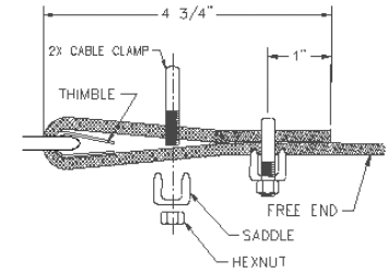
Diagram 10A. Saddling the cable on one end.
