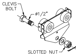
Diagram 6A. Installing hoist on 250# hoist trolley.
