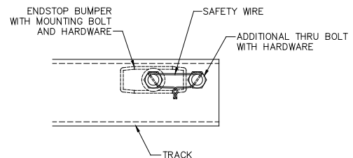
Diagram 10E. Double wired end stop.
