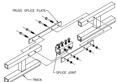
Diagram 4D. Splicing tracks together.
