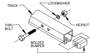
Diagram 10D. Installing endstop.
