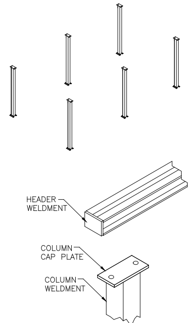
Diagram 2A. Orienting column cap plate.
