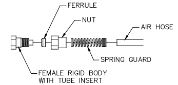
Diagram 10F. Female fitting assembly.
