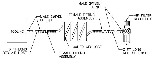
Diagram 10G. Coiled air hose assembly.
