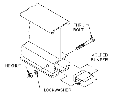
Diagram 5F. Installing end stop.
