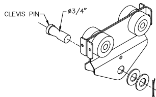
Diagram 6B. Installing hoist on 500# hoist trolley.
