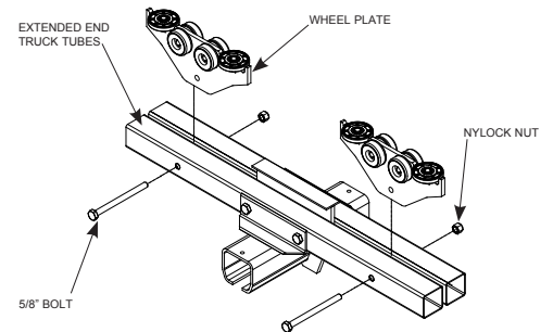
Diagram 5C. Installing wheel plates.
