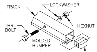
Diagram 4F. Installing end stop.
